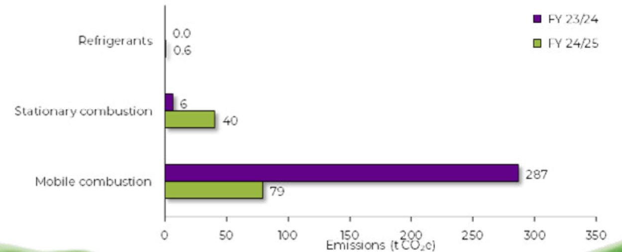
Figure 4: Graphical representation for the quantified emissions for Scope 1 as per the GHG Protocol categories for the Group in the FY 2023/24 in comparison to this reporting year 2024/25.
